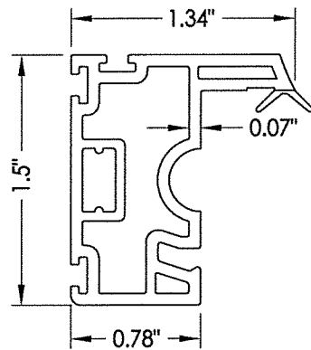
5 STILE/RAIL
