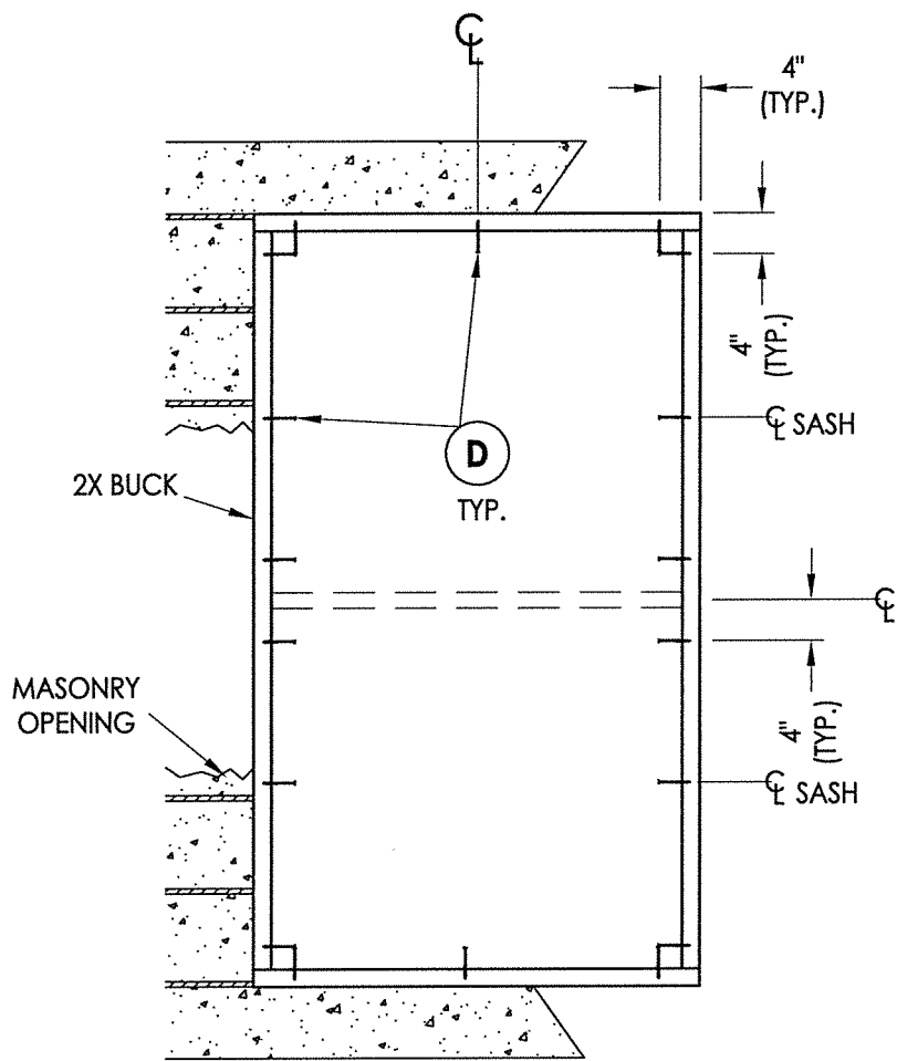
BUCK ANCHORING
