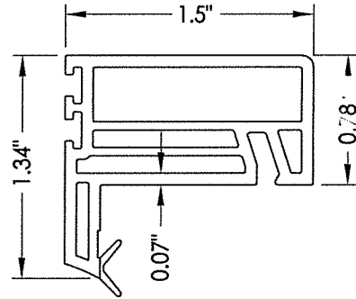
7 LOCK RAIL
