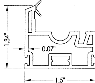
6 KEEPER RAIL
