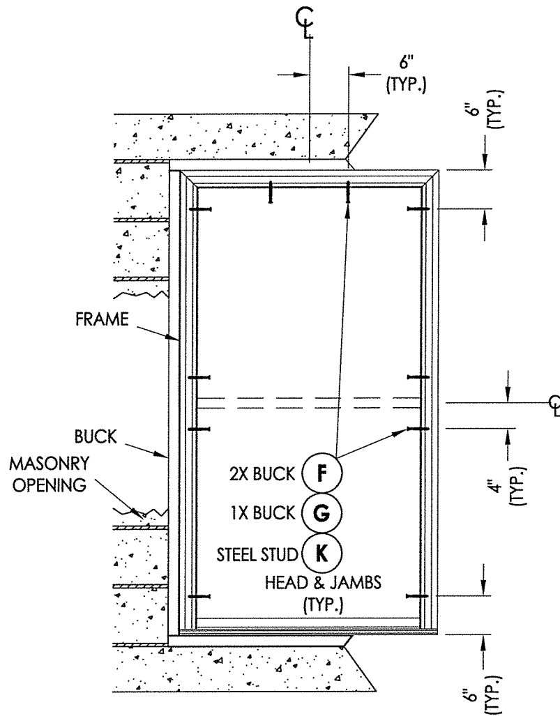
FRAME ANCHORING
